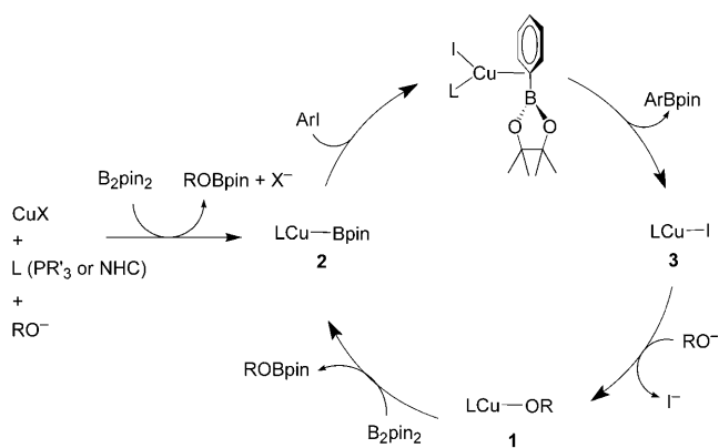
Scheme 1. A possible, simple catalytic cycle for the copper-catalyzed borylation of aryl halides.
